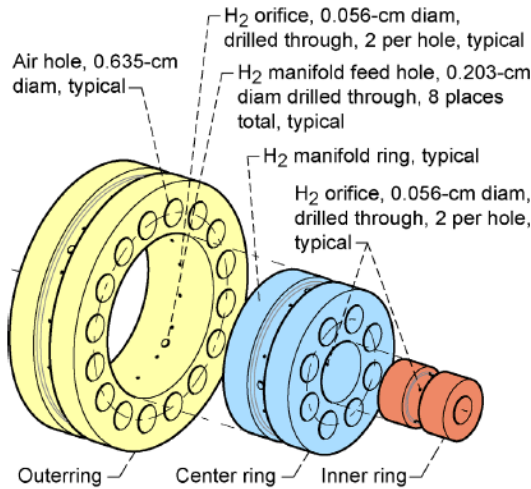
Figure 2. Three-piece injector brazing assembly detail—25 air holes total [21].
