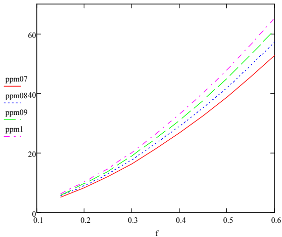
Figure 9. NOx emissions [ppm] depending on the equivalence ratio at T_3=800\text{ K} , p_3= 0.7, 0.8, 0.9, 1\text{ MPa} A^*=14 (advanced LDI technology)
