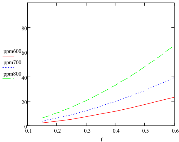
Figure 4. NOx emissions [ppm] depending on the equivalence ratio at p_3=1\text{ MPa=ct} , T_3=600, 700, 800\text{ K}
