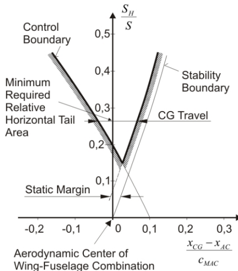
Fig. 9 – Horizontal tail sizing scissor plot showing the forward and aft CG boundaries from control and stability requirements and the required CG range
